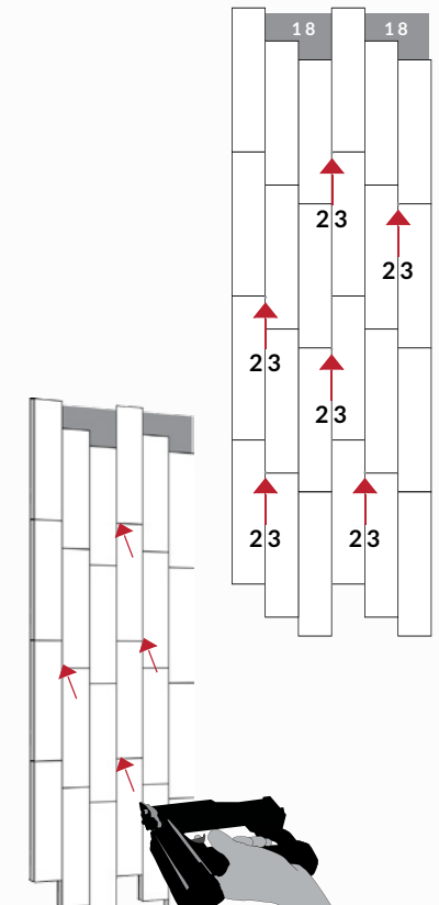
FIG. C BELOW EYE LEVEL, USE #23 GAUGE NAILS, NAILING AT AN UPWARD ANGLE TO AVOID VISIBLE NAILS.
