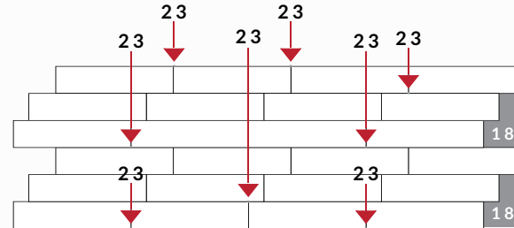
FIG. A: ABOVE EYE LEVEL, USE #23 GAUGE NAILS AT A DOWNWARD ANGLE.
