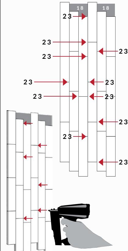
FIG. B AT EYE LEVEL, USE #23 GAUGE NAILS, NAILING INTO THE EDGES OF EACH PANEL.
