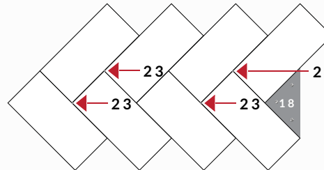
FIG. B: AT EYE LEVEL, USE #23 GAUGE NAILS, NAILING INTO THE EDGES OF EACH PANEL.
