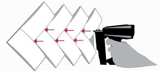
FIG. B: AT EYE LEVEL, USE #23 GAUGE NAILS, NAILING INTO THE EDGES OF EACH PANEL.
