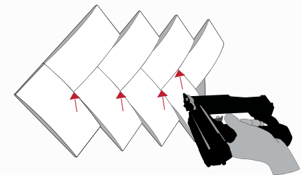
FIG. C: BELOW EYE LEVEL, USE #23 GAUGE NAILS, NAILING AT AN UPWARD ANGLE TO AVOID VISIBLE NAILS.
