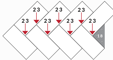
FIG. A: ABOVE EYE LEVEL, USE #23 GAUGE NAILS AT A DOWNWARD ANGLE.
