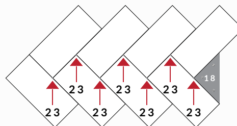
FIG. C: BELOW EYE LEVEL, USE #23 GAUGE NAILS, NAILING AT AN UPWARD ANGLE TO AVOID VISIBLE NAILS.
