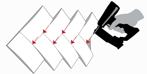
FIG. A: ABOVE EYE LEVEL, USE #23 GAUGE NAILS AT A DOWNWARD ANGLE.
