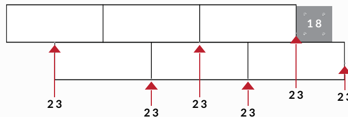
FIG. C: BELOW EYE LEVEL, USE #23 GAUGE NAILS, NAILING AT AN UPWARD ANGLE TO AVOID VISIBLE NAILS.
